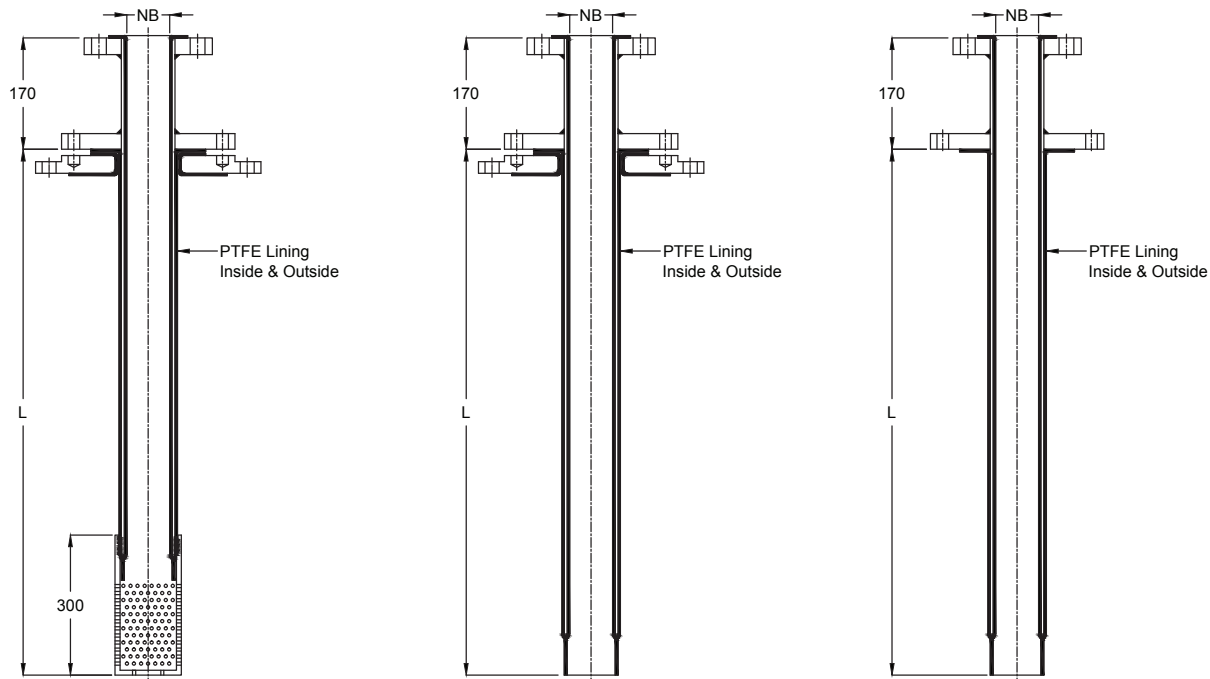
Dimension detail for Straight Dip Pipe
